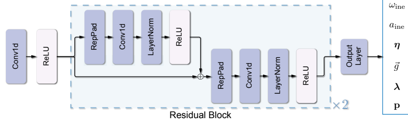
Fig. 3. The detailed architecture of DyNet.
