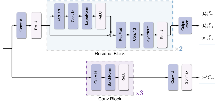
Fig. 4. The detailed architecture of attentive PD controller.
