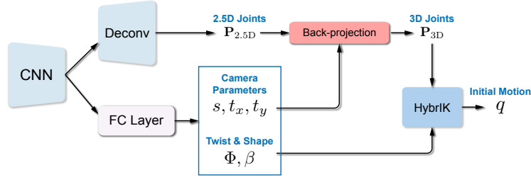
Fig. 2. The detailed architecture of the kinematics backbone.
